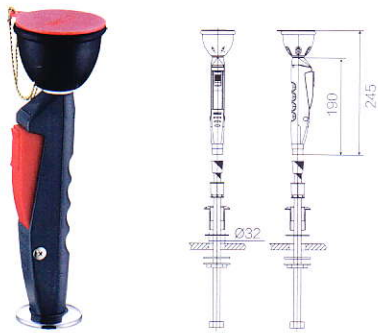
WJH1355-1 台式移动单口洗眼器 Removable Single Nozzle Eye Wash(table mounted)
